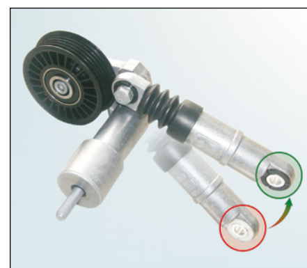
Figure 2: 534 0014 10 - Version showing both black and white plastic bushes on hydraulic damper
