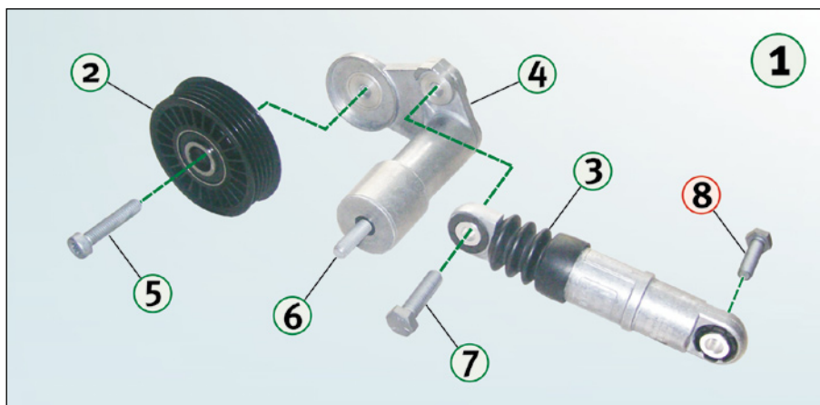
Figure 1: Detailed illustration of 534 0014 10 including all components
